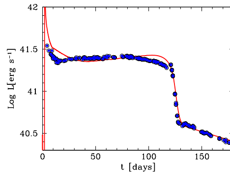
Fig. 2. Bolometric light curve of SN 2008bk (blue circles) and hydrodynamic model (red line). The horizontal axis shows the time since explosion.
