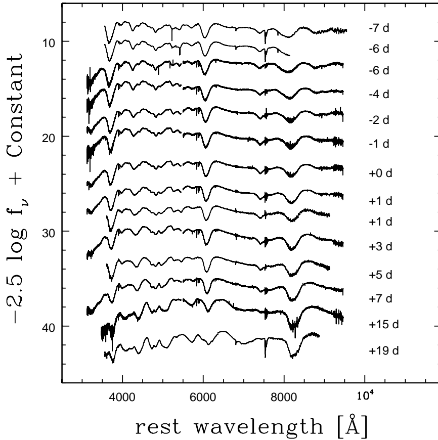
Fig. 3. Spectroscopic sequence of the Type Ia SN 2010ev, covering the first 26 days of its evolution. Each spectrum is labeled with the time since maximum light. The spectra were obtained with the VLT/XSHOOTER, Gemini-South/GMOS and Magellan instruments.
