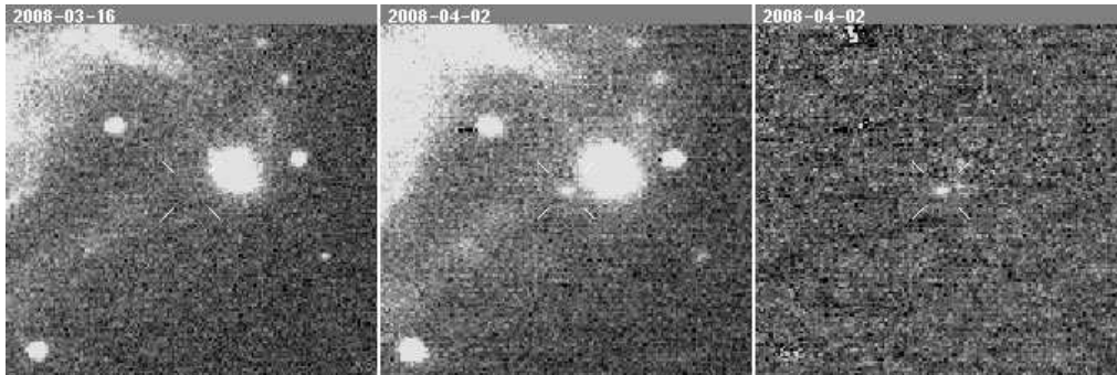
Fig. 1. An example of the three images generated by the pipeline. On the left is the pre-discovery image, in the middle is the new image, and in the right is shown the difference image. In this case the new object corresponds to SN 2008bp.
